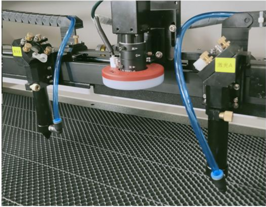
Multi Heads
